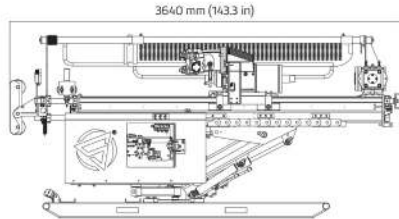
Levent 3003 Skid
